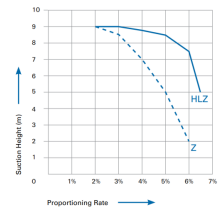
Suction Height vs. Proportioning Rate
