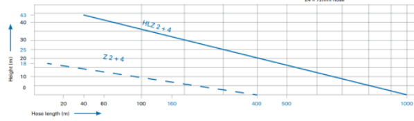
Operating Height vs. Hose Length
