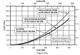
PRESSURE LOSS
