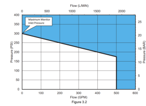
OPERATING ENVELOPE
