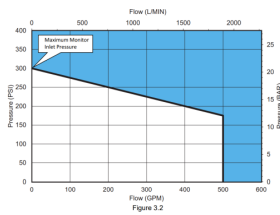
OPERATING ENVELOPE
